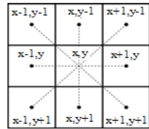
Fig. 4. Local configuration for computing the intensity variation at (x, y) .
