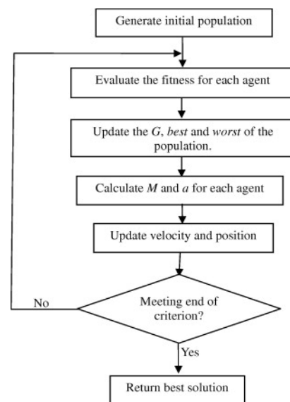
Fig. 2. Flowchart of gravitational search algorithm.
